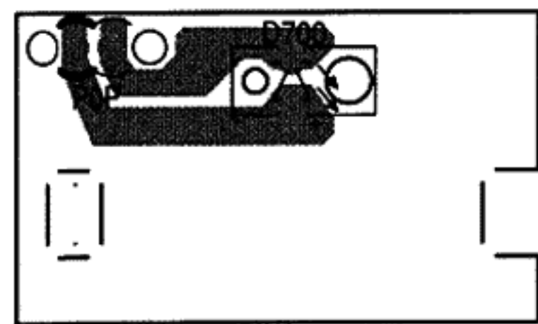
Power-LED -Platte / Power LED Board
