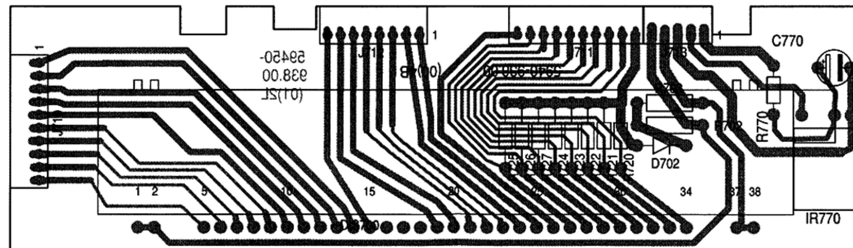
Displayplatte / Display Board
