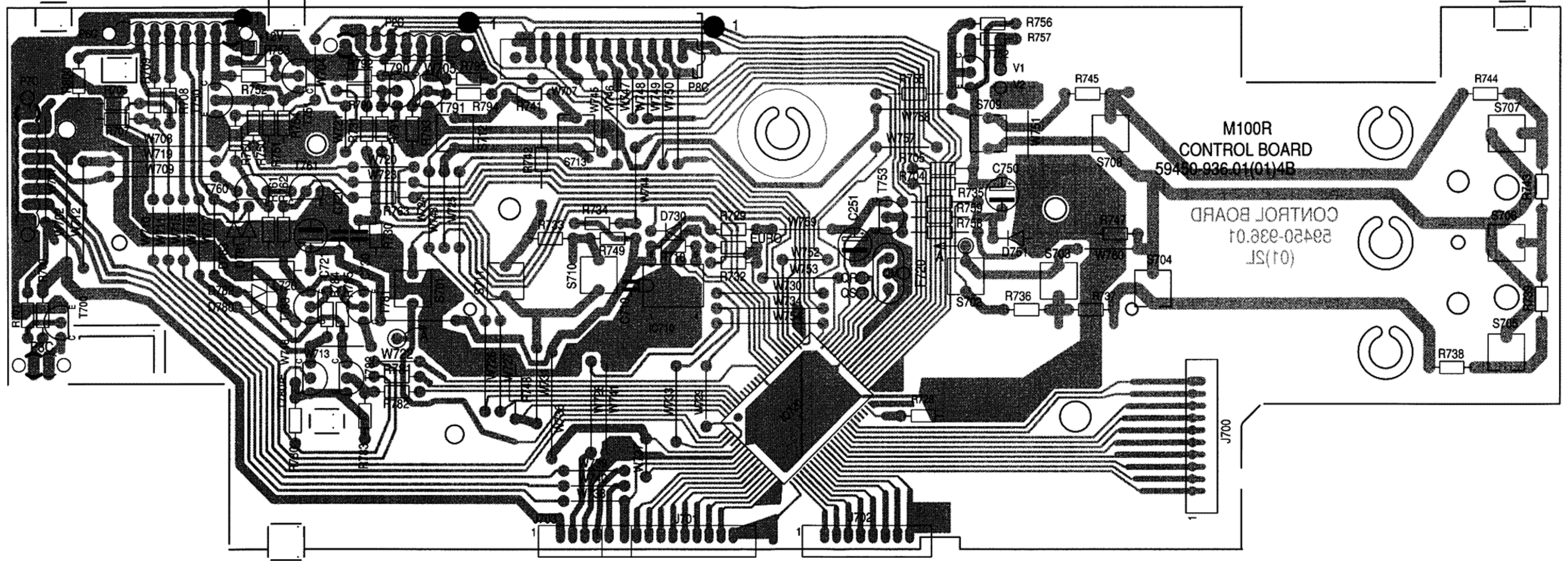
Bedienplatte / Control Board
