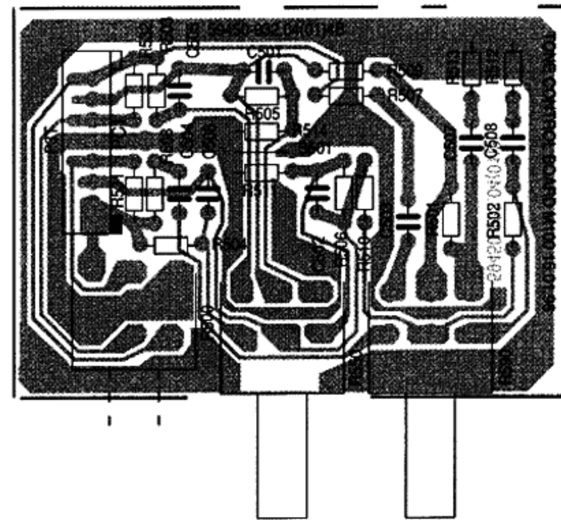
Klangreglerplatte / Tone Control Board
